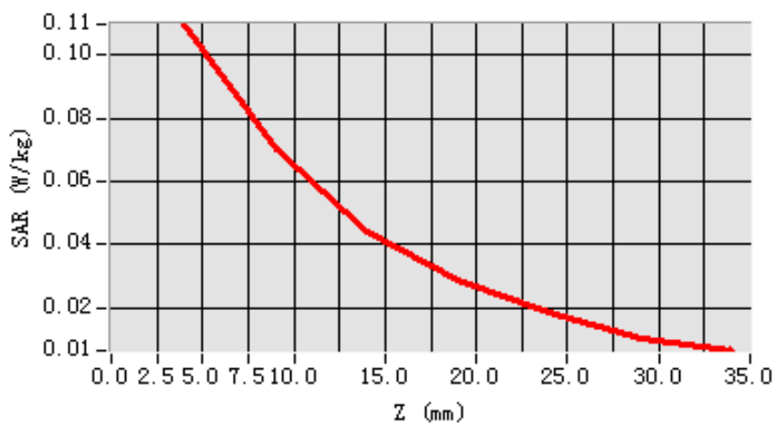
SAR, Z Axis Scan (X = -47, Y = -56)
