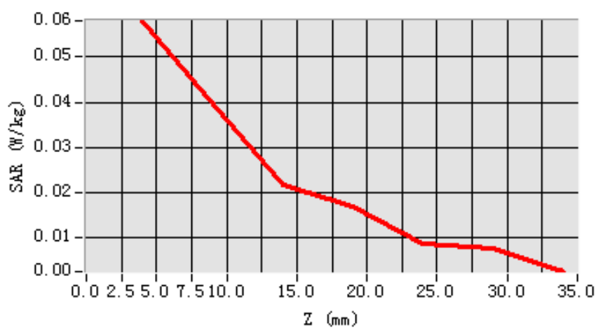
SAR, Z Axis Scan (X = -41, Y = -55)
