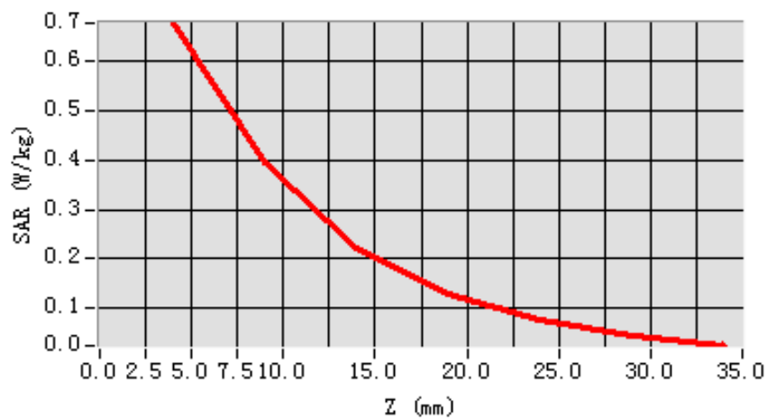
SAR, Z Axis Scan (X = -55, Y = -60)
