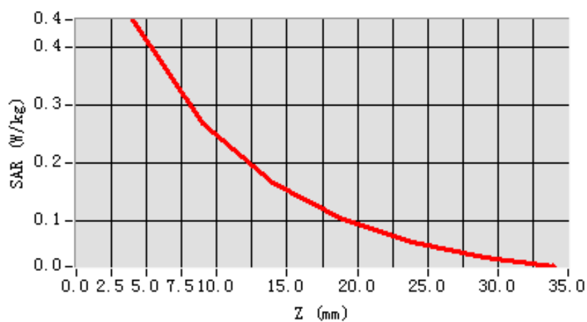
SAR, Z Axis Scan (X = -50, Y = -64)
