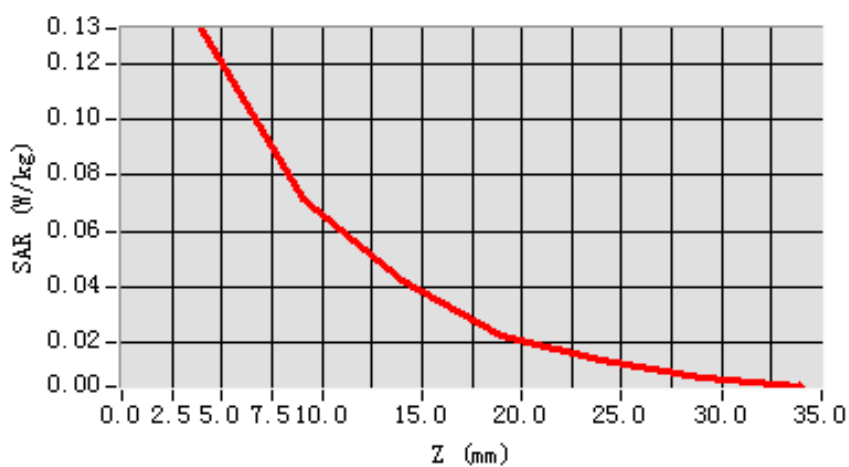
SAR, Z Axis Scan (X = -40, Y = -48)
